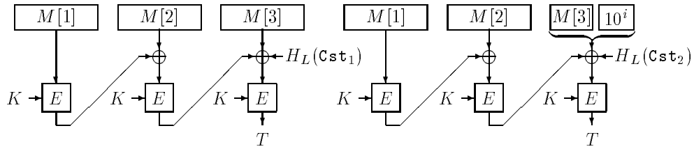
Figure 4: Illustration of OMAC-family.
