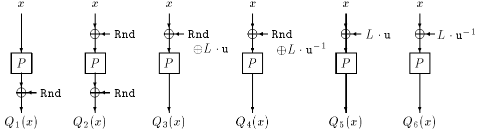
Figure 6: Illustrations of Q_1, Q_2, Q_3, Q_4, Q_5 and Q_6 . Note that L = P(\mathbf{Cst}) .
