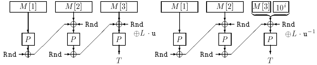
Figure 11: Computation of \mathcal{B}_{\mathcal{A}} when \mathcal{O}_i = Q_i for 1 \leq i \leq 6 , and |M| > n .
