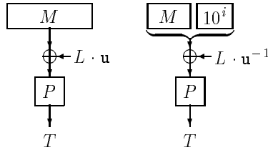
Figure 12: Computation of \mathcal{B}_{\mathcal{A}} when \mathcal{O}_i = Q_i for 1 \leq i \leq 6 , and |M| \leq n .
